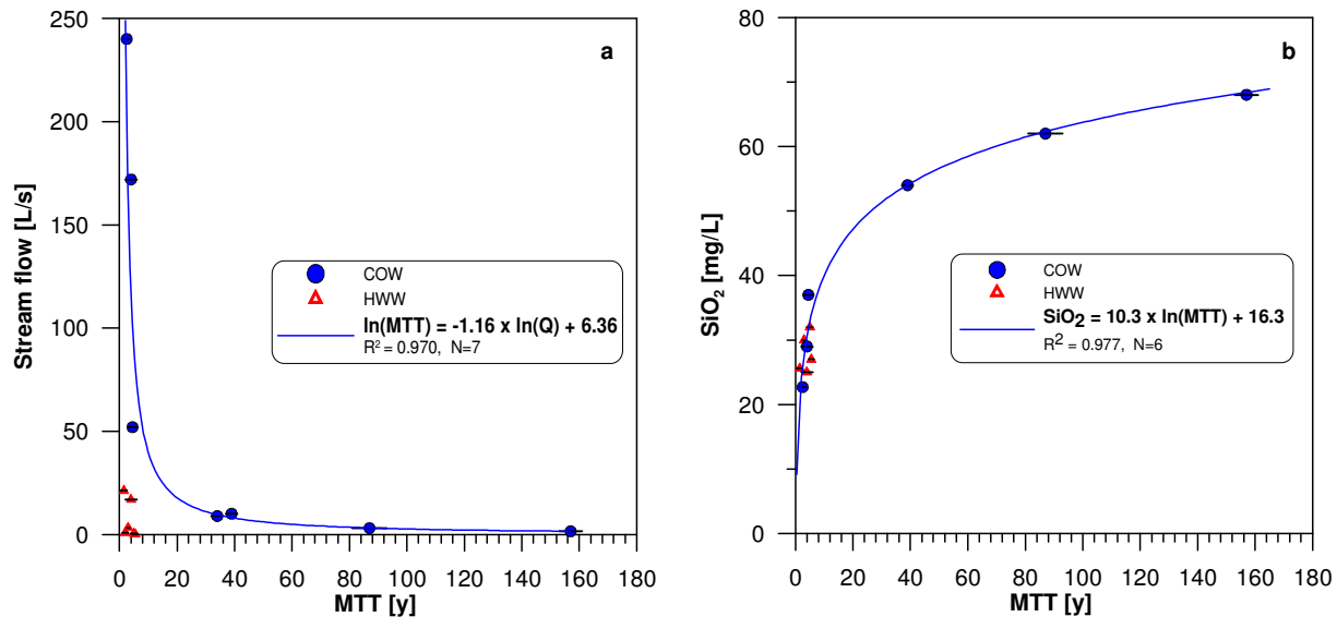
Fig. 7. (a) Streamflow and (b) SiO 2 concentration versus mean transit time (MTT). Correlations are deduced from data from the catchment outflow weir (COW) only.
