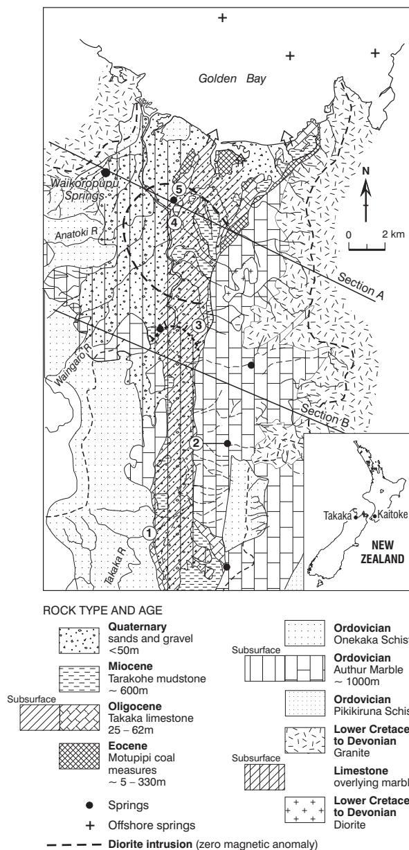
Fig. 1. Hydrogeological map of the Takaka Valley, NW Nelson, New Zealand (modified from Ford and Williams, 1989). Note the zero magnetic anomaly outline (inferred diorite intrusion).
